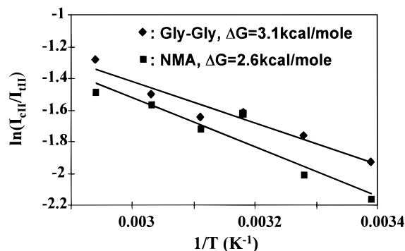
Figure 4. Natural log of the ratio of the cis amide II to the trans amide II band Raman intensities as functions of 1/T . The solid lines are the best linear least-square fit whose slope give the Gibbs free energy gap between the cis and trans amide forms.
