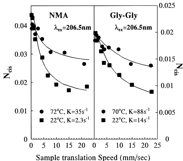
Figure 7. Concentration of cis -NMA and cis -Gly-Gly as a function of sample translation speed (206.5 nm excitation). The solid curves are the least-squares best fit based on the three-state model, which extracts the isomerization rates from the cis to the trans forms.
